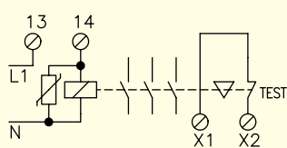
Controlled monitoring of external contactor, relay, valve or JOKAB SAFETY's expansion relays.
