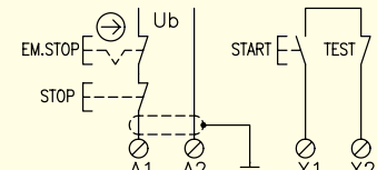
JSBT5 as emergency stop and control relay with Start and Stop function.
